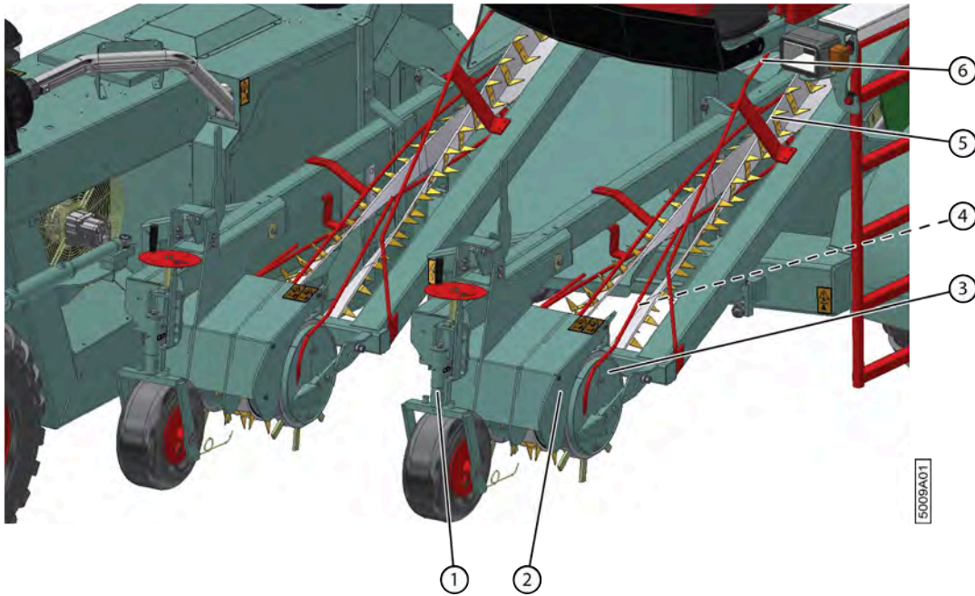
Fig. 42: Pick-up
