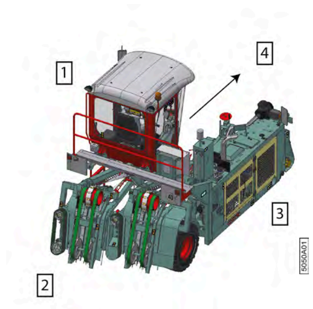
Fig. 7: Direction
